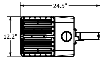
LED Fixture Top view
